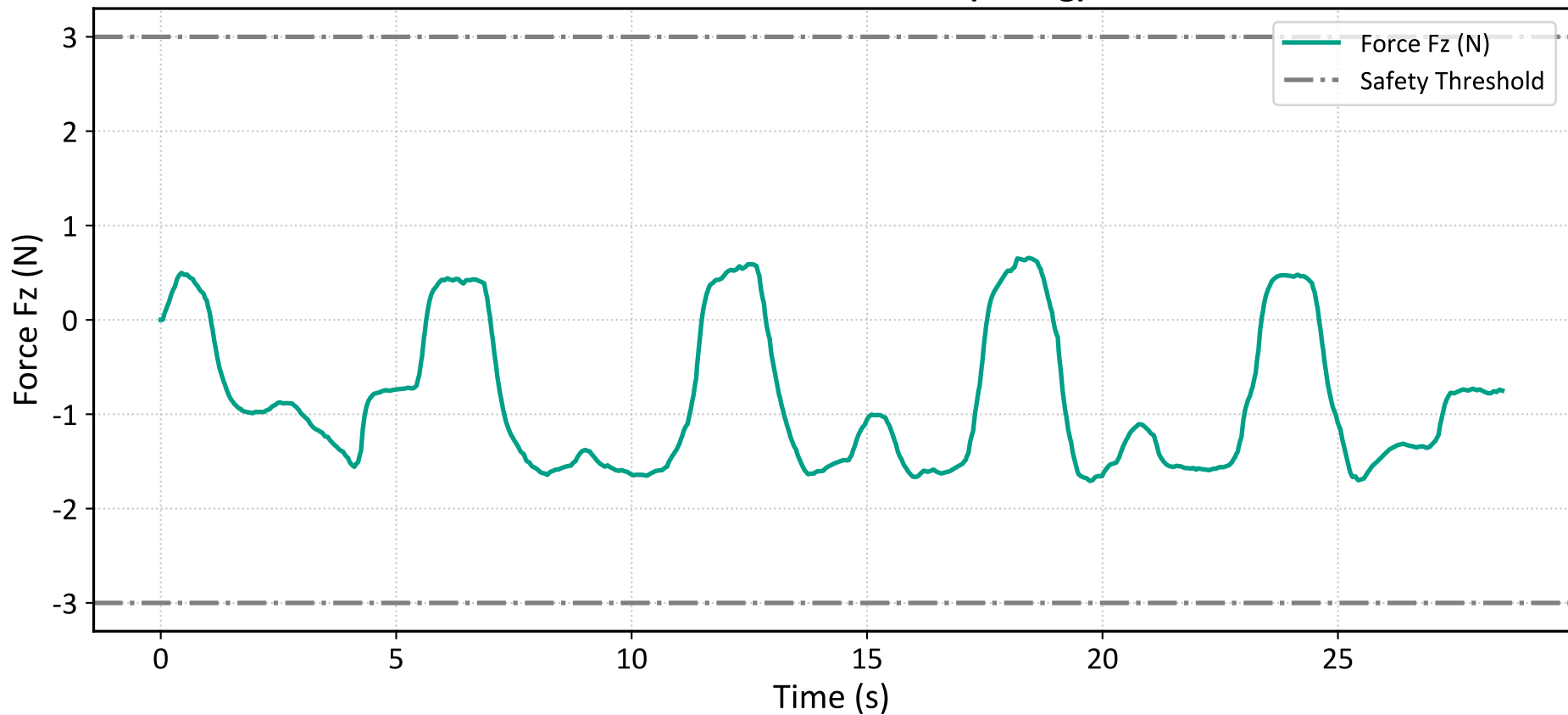
Interaction Force Profile (Lifting)
